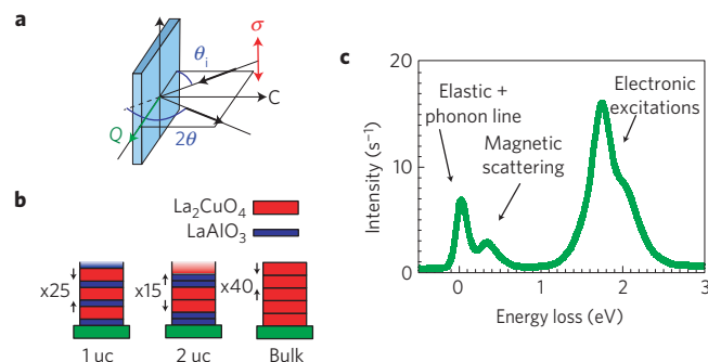
Figure 1 | The scattering geometry, a schematic of the samples and a typical RIXS spectrum. a , The experimental scattering geometry. The 931 eV \sigma -polarized X-rays are incident at an angle \theta_i and are scattered through a fixed angle 2\theta = 130^\circ . Large \mathbf{Q} corresponds to near-grazing incidence ( \theta_i \rightarrow 0 ). b , The multilayer films studied, composed of 13.2 Å \text{La}_2\text{CuO}_4 layers (red blocks) containing two \text{CuO}_2 planes and 3.8 Å \text{LaAlO}_3 (blue blocks). We label the films, on the basis of the thickness of \text{La}_2\text{CuO}_4 , as 1 uc, 2 uc and bulk. The arrows denote the repeat unit of the films ( \times 25 , \times 15 , \times 40 ). c , A representative RIXS spectrum of the 1 uc \text{La}_2\text{CuO}_4 film ( 25 \times [\text{LaAlO}_3 + \text{La}_2\text{CuO}_4] ) at \mathbf{Q} = (0.77\pi, 0) identifying the main spectral features: the elastic and phonon scattering around zero-energy transfer, the magnetic scattering around 300 meV and the electronic ( dd ) excitations from 1 to 3 eV.
