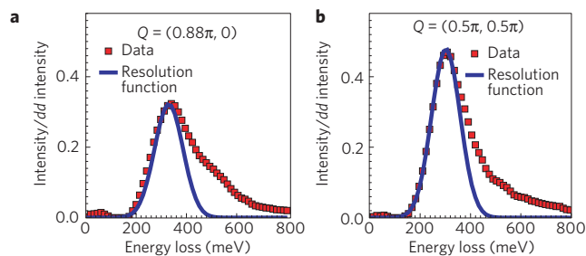
Figure 3 | Magnon peak showing anisotropic high-energy magnetic scattering. a, b , The measured magnetic spectral weight (red squares) in bulk \text{La}_2\text{CuO}_4 at \mathbf{Q} = (0.88\pi, 0) (a) and \mathbf{Q} = (0.5\pi, 0.5\pi) (b) . The blue line is a resolution-limited Gaussian at the single-magnon energy. The statistical error bars are smaller than the point size.
