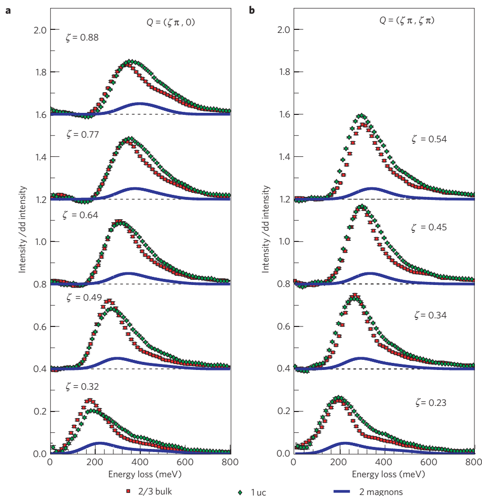
Figure 4 | Scaling of the magnetic excitations. a,b , A comparison between 2/3 of the bulk \text{La}_2\text{CuO}_4 response (red squares) and the 1 uc ( 25 \times [\text{LaAlO}_3 + \text{La}_2\text{CuO}_4] ) response (green diamonds) along (\zeta\pi, 0) ( a ) and (\zeta\pi, \zeta\pi) ( b ). The difference between these spectra corresponds to the longitudinal magnetic response, to be compared to the two-magnon S^{zz}(\mathbf{Q}, \omega) calculation (blue line) 22 . As it is not possible to measure absolute magnetic scattering intensities with RIXS at present, the calculation is shown with an arbitrary intensity.
