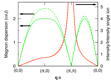
FIG. 3 (color online). Momentum dependence of the magnetic RIXS spectral weight at the copper L_3 edge (red) and the magnon dispersion (green) for a simple 2D Heisenberg model (solid lines) and an extended model relevant for \text{La}_2\text{CuO}_4 [24] (dashed).
